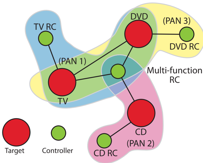
Figure 1 - Example ZigBee RF4CE network topology
