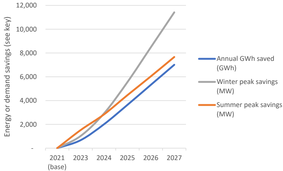
Figure ES-1. Cumulative annual energy and peak savings by year from the sum of the seven programs analyzed
