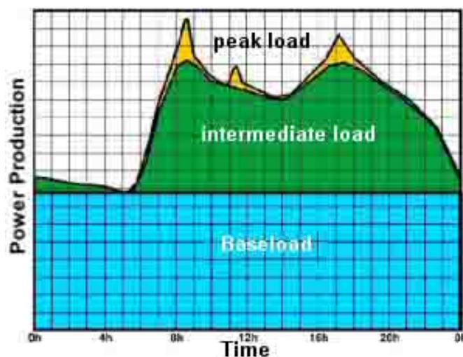
Figure 1. Schematic of base, intermediate and peak load. This shows a typical winter day. Source: Wind Watch 2021. Demand response programs help curtail the need for peak load generation, while energy efficiency programs lower the need for baseload or intermediate load generation.
