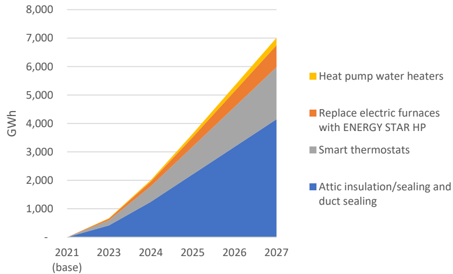
Figure 5. Energy savings (GWh) by program and year
